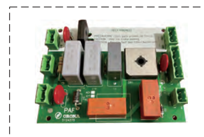
5124375 Orona elevator pcb
