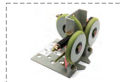
C0083111 - B/16501278 - A Hitachi roller guide shoe
