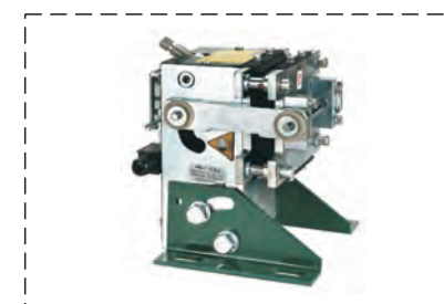
OX - 250 Elevator wire rope brake
