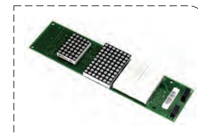
ID.NR.59324318 Schindler display board
