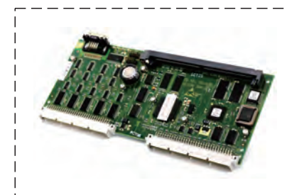
ID.NR.591640 Schindler 5400 main board
