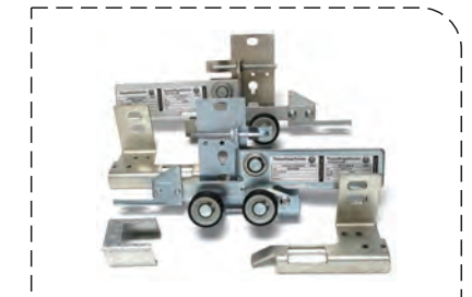
M2Z(T)S8 TKE elevator door lock
