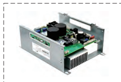
LRU - 403(ACD4 - MR) Otis elevator inverter
