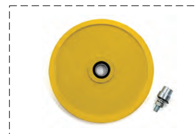
250*20*6005 Otis governor tension wheel
