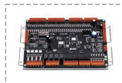
KLS-MCU Canny main board
