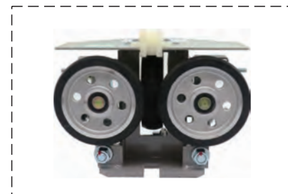
RG150 Kone roller guide shoe
