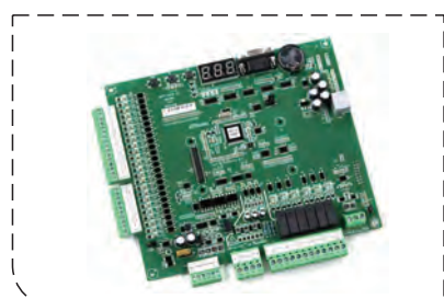
MCTC-MCB-C2/C3/B/G Monarch main board
