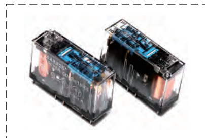
G7SA-3A1B Omron salay relay
