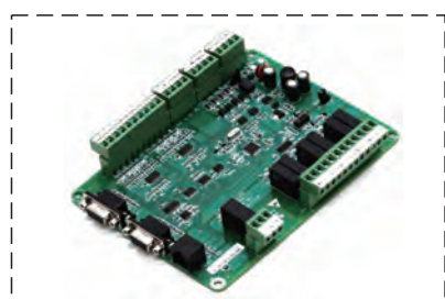
MCTC-CTB-A/B Monarch car top board
