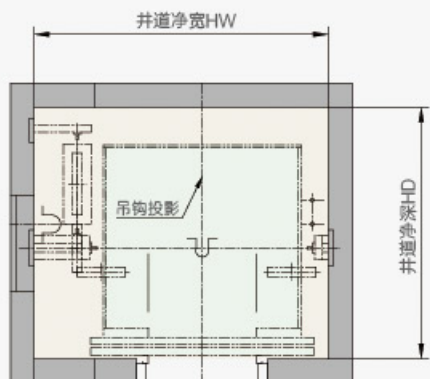
顶层平面布置图 TOP-FLOOR PLANAR GRAPH
