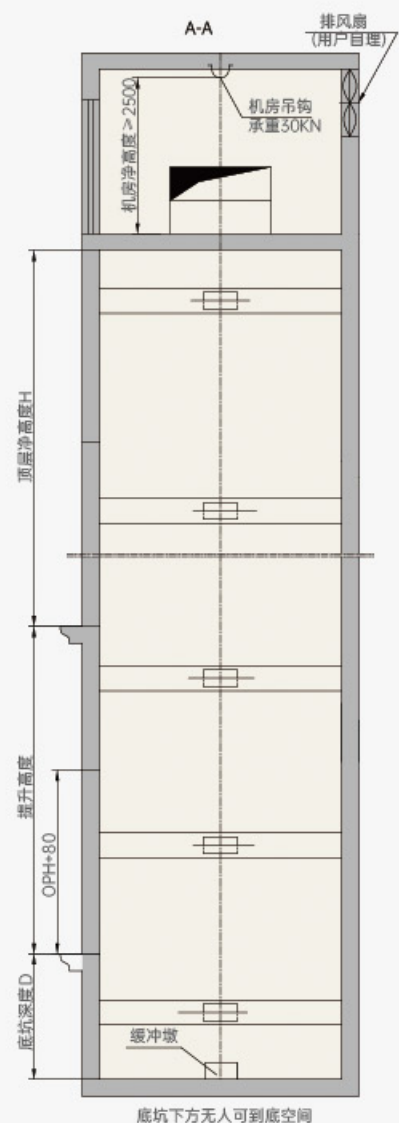
A-A井道纵剖面图 A-A WELL AND VERTICAL SECTION DIAGRAM
