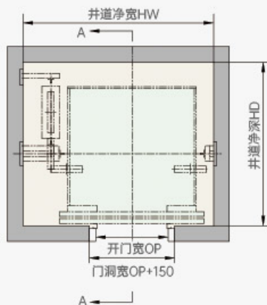
井道平面图 WELL ROAD PLAN
