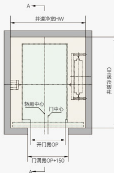
井道平面图 WELL ROAD PLAN
