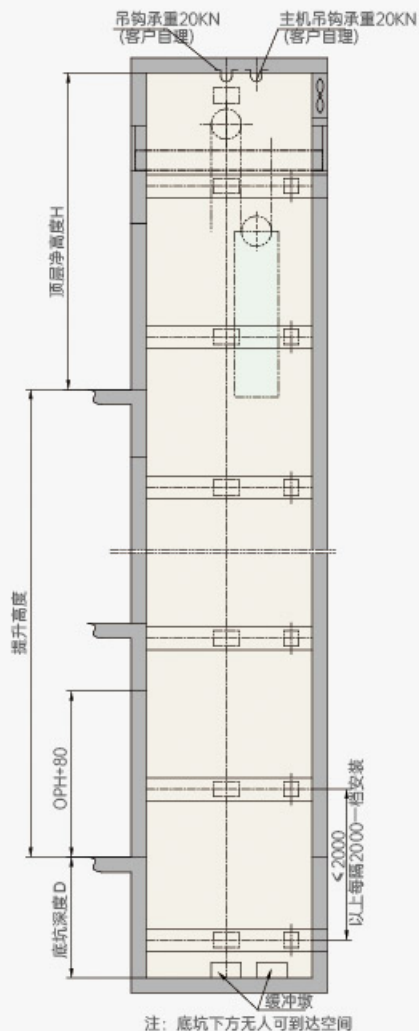
A-A井道纵剖面图 A-A WELL AND VERTICAL SECTION DIAGRAM
