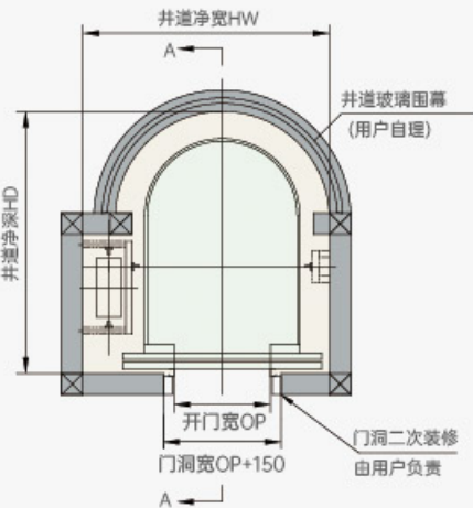
井道平面图 WELL ROAD PLAN
