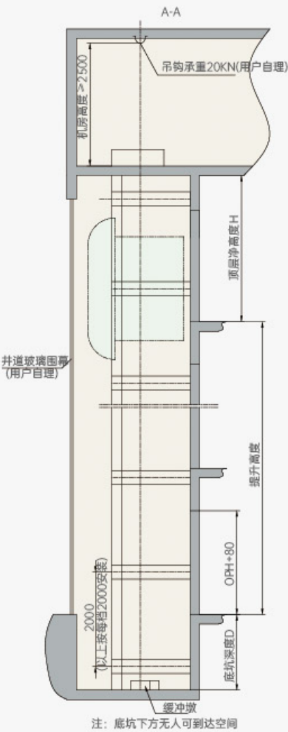
A-A井道纵剖面图 A-A WELL AND VERTICAL SECTION DIAGRAM
