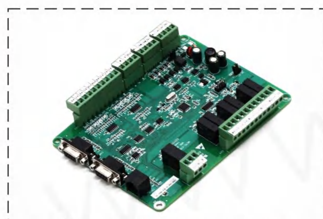
MCTC-CTB-A/B Monarch car top board
