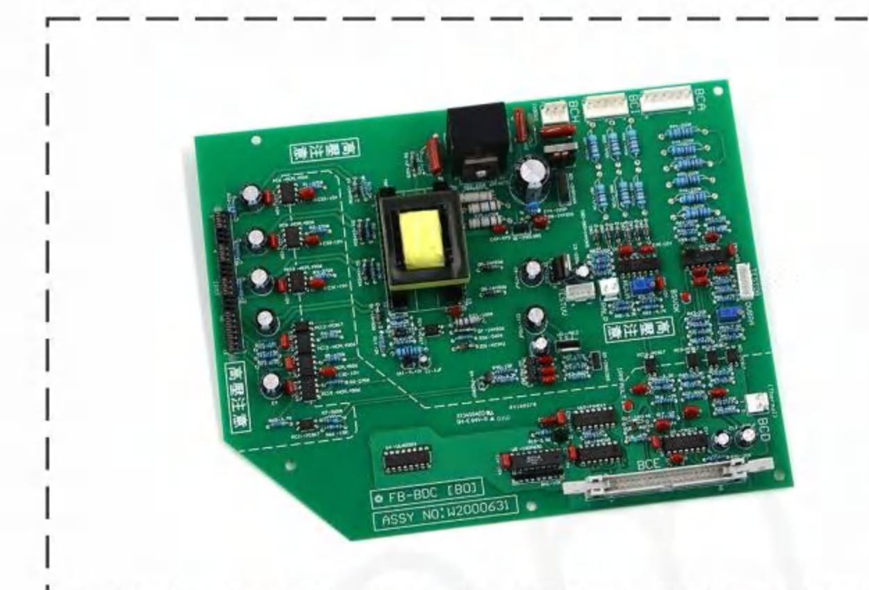
DC006482 W2000631 Yungtay drive board
