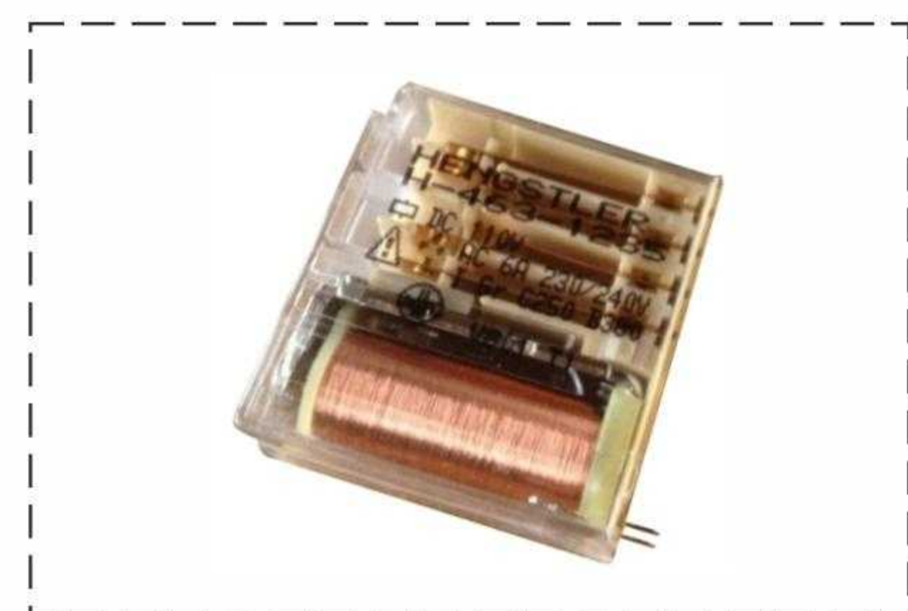
H-463-1212 Hengstler safety relay
