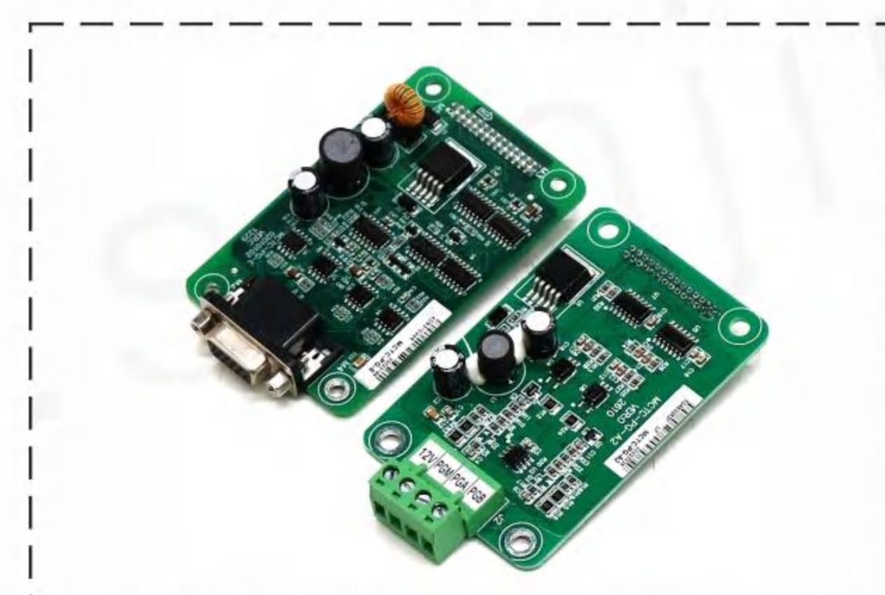
MCTC-PG-E/A2 Monarch pg card
