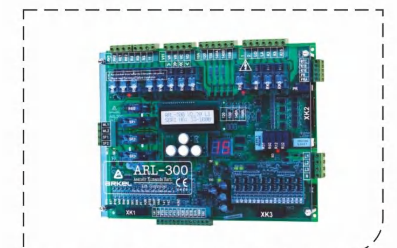
ARL-300/500 Arkel control board
