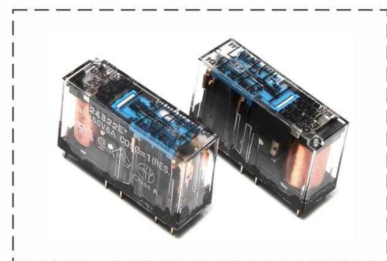
G7SA-3A1B Omron salay relay
