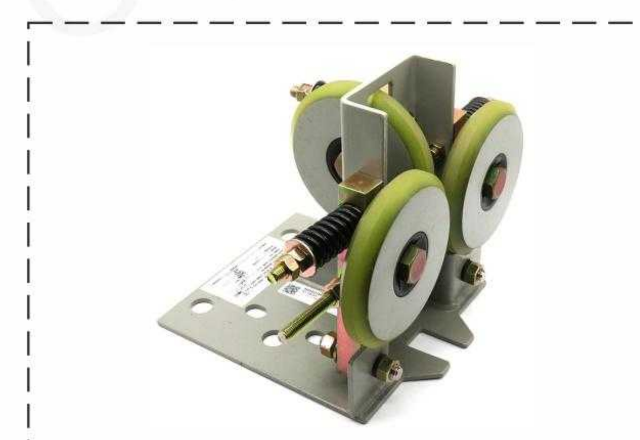
C0083111-B/16501278-A Hitachi roller guide shoe
