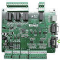
MCTC-CTB-A CANbus connection via main control board
