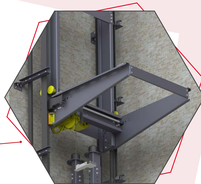
SPECIAL SPEED GOVERNOR
