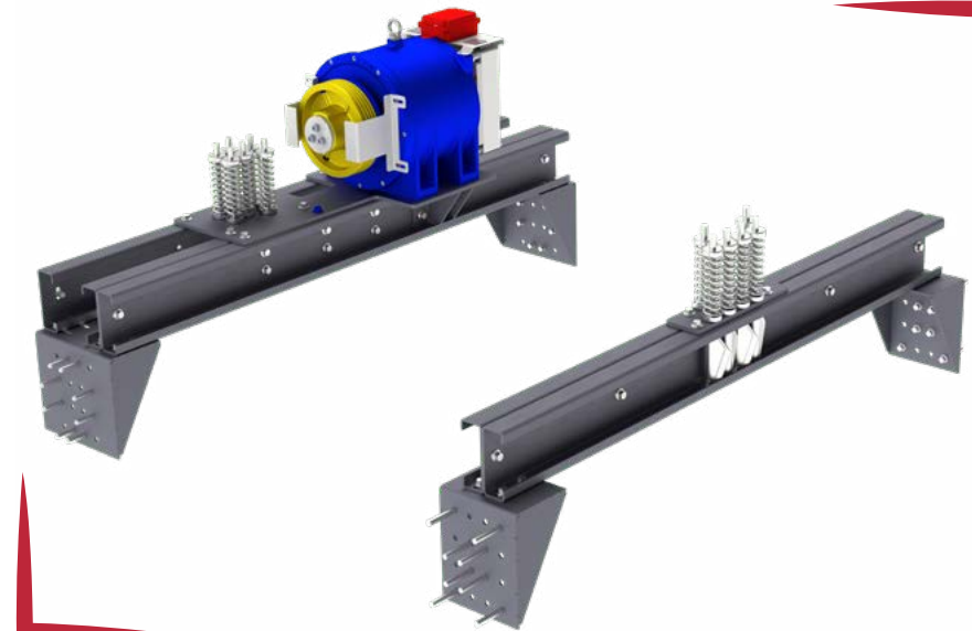
MRL. MACHINE MOTOR FRAME
