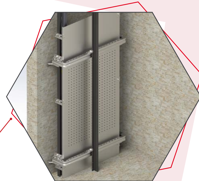
SIPARATION METAL SHEET
