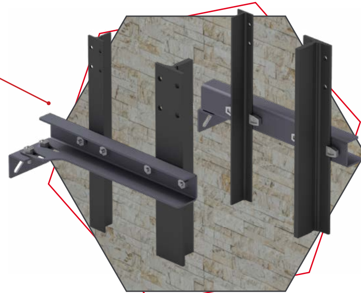
L TYPE CAR FRAME BRACKET
