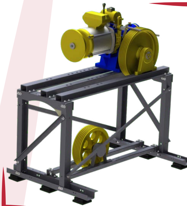
MR. MACHINE MOTOR FRAME
