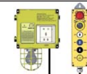
Emergency stop Monarch MCTC00-JP-P6Y-02 UP002036
