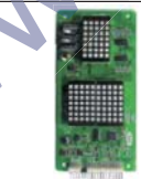
Elevator board Monarch MCTC-HCB-R1 UP000633
