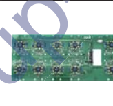
Elevator board Toshiba UCE13-68C UP002585
