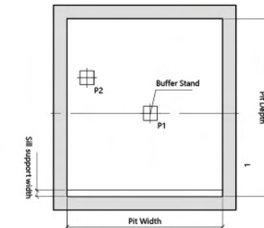
Pit Plan View/1:60
