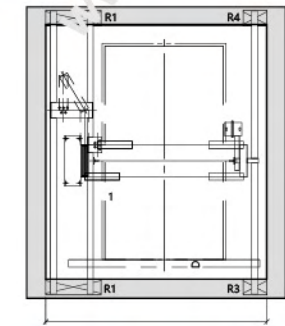
Shaft Plan View/1:60
