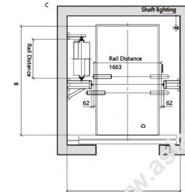
Pit Plan View/1:60
