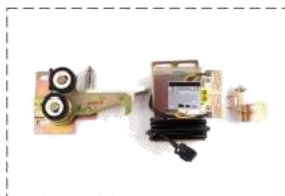
STVF7/STVF9 Hyundai door lock device
