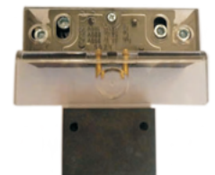
东芝付锁AZ-05 SP000063 Toshiba elevator female lock
