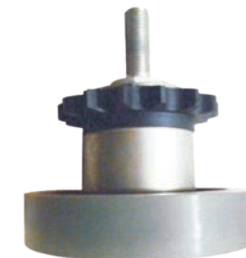
日立新式驱动轮总成 SP02220 HITACHI Driving wheel assembly (New type)
