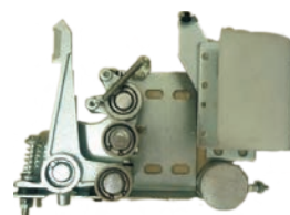
通用06门锁SP001095 General elevator door lock
