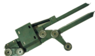
三菱161门刀SP001073 Mitsubishi elevator door clutch
