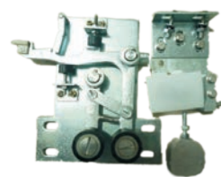
货梯PB16D门锁(右)SP000382 cargo elevator door lock
