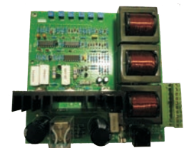
门机调速板 Door Machine speed regulation PCB XDMJ-TS110 sp4692
