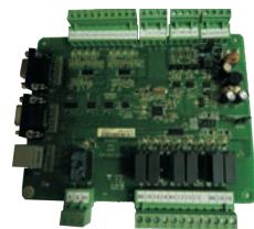
轿顶通讯板 ceiling assembling messgae board MCTC-CTB-A SP4215
