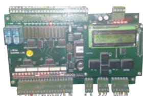
莱茵电梯主板 Rhein Main Board LME66 SP4043
