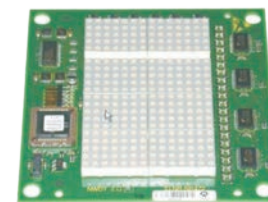
迅达显示板 ID NR591472 Schindler display Board ID Nr591472
