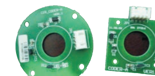
康力电梯门机编码器 canny-elevator Door encoder sp4580
