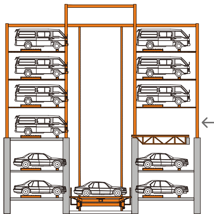
Half-underground plan
