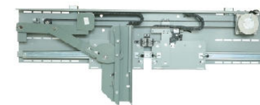
·GF-MP-211 Center Opening Two Panel Operator (Car Frame Installation)
