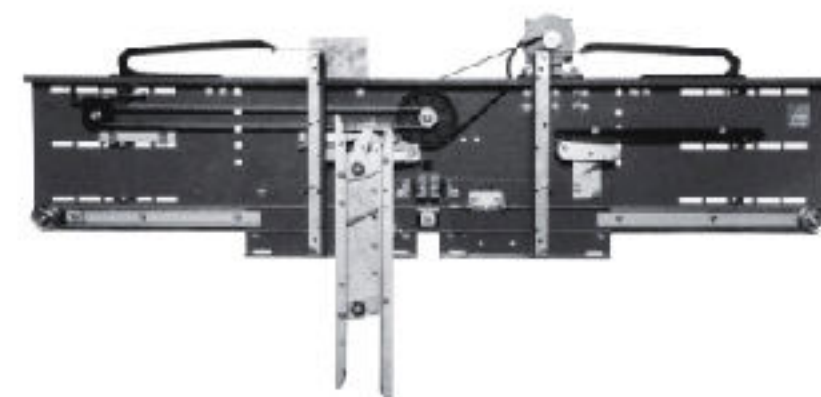
·GF-131-50B Center Opening VVVF Door Operator (Car Top Installation)
