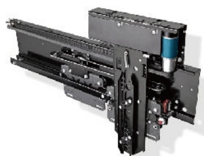
·GF-ECO-12/R-L Two Panels Telescopic Opening Car Door Operator
