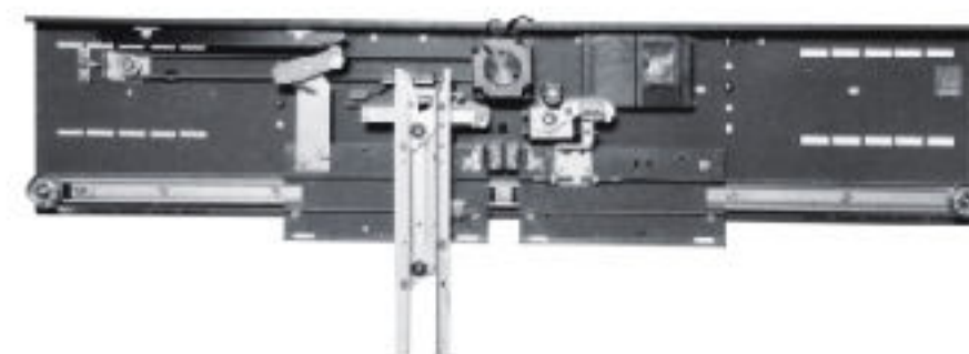
·GF-131-50-YC-B Center Opening AC PM Door Operator (Car Top Installation)
