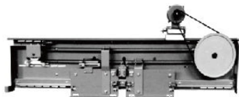
·GF-131-06B Center Opening VVVF Door Operator (Car Top Mounting)
