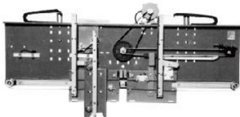
·GF-131-50-1B Center Opening VVVF Door Operator (Car Top Installation)
