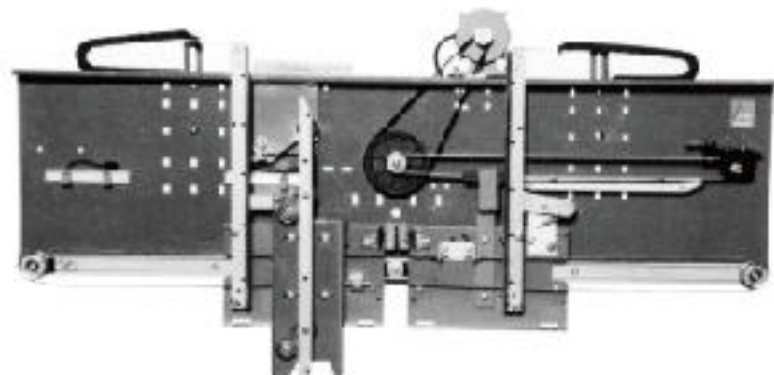
·GF-131-50-1A Center Opening VVVF Door Operator (Straight Beam Mounting)
