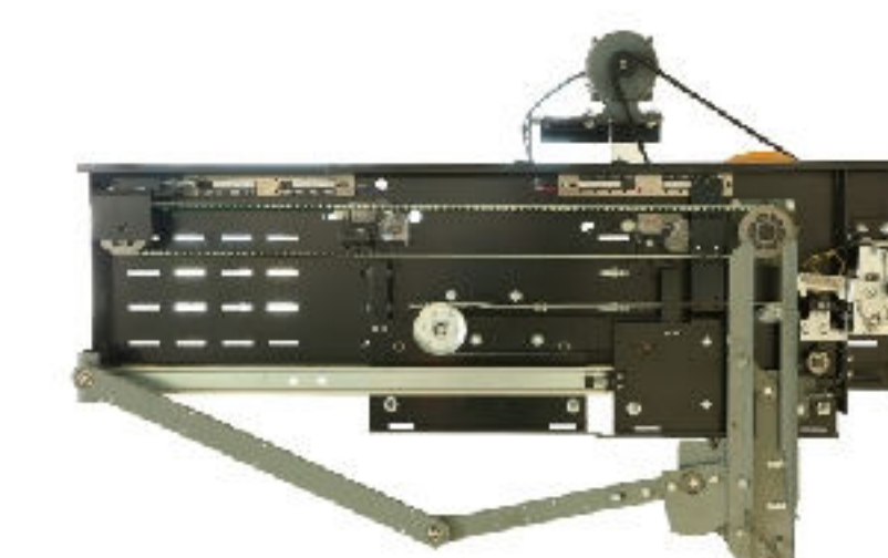
·GF-MVT-211 Side Opening Two Panel Operator (Car Frame Installation)
